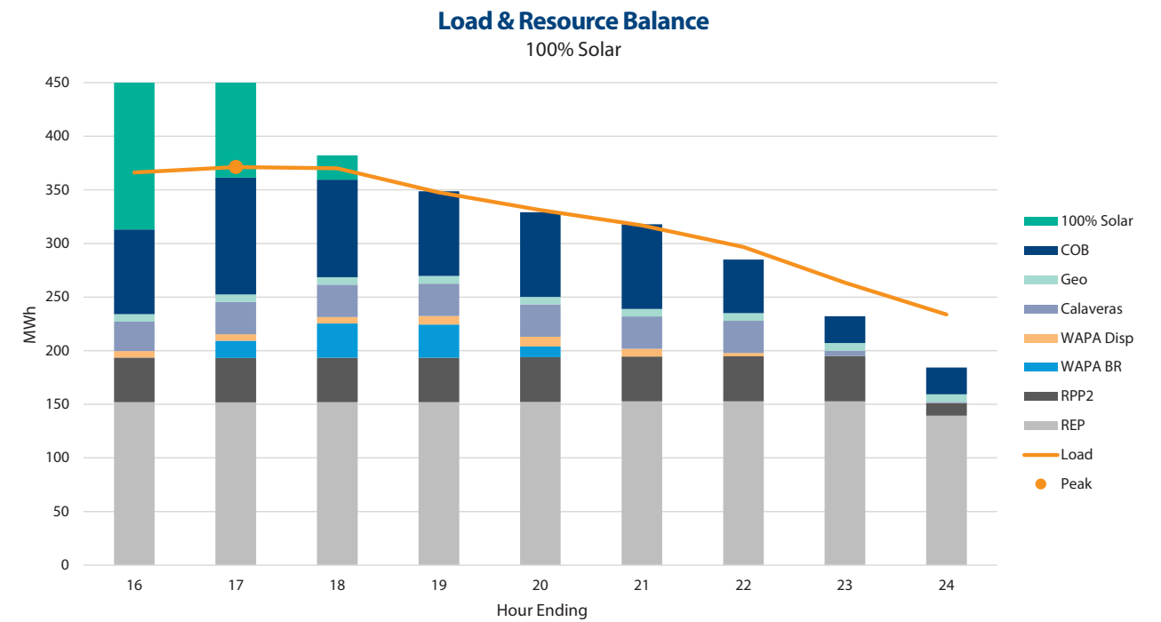
Figure 53: Load and Resource Balance on September 6, 2022 using the 100% Solar Portfolio
